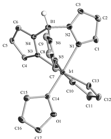
Figure 2. ORTEP view of complex 6 . Thermal ellipsoids are set at 30% probability level. Selected bond lengths [Å] and angles [°]: Ir1–C10 2.051(6), Ir1–C13 2.033(6), Ir1–C14 1.898(6); C10–Ir1–C13 80.7(3).
