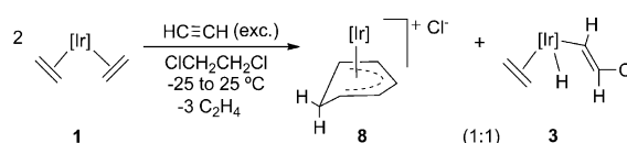
Scheme 6. Reaction of complex [\text{TlIr}(\text{C}_2\text{H}_4)_2] ( 1 ) with acetylene in 1,2-dichloroethane.
