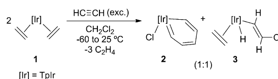
Scheme 2. Reaction of complex [\text{TlIr}(\text{C}_2\text{H}_4)_2] ( 1 ) with acetylene in \text{CH}_2\text{Cl}_2 .
